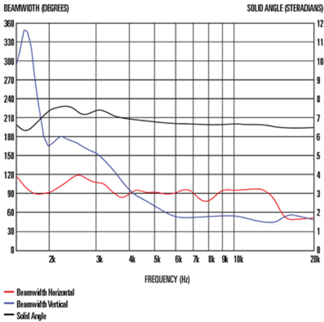
Beamwidth and Solid Angle
