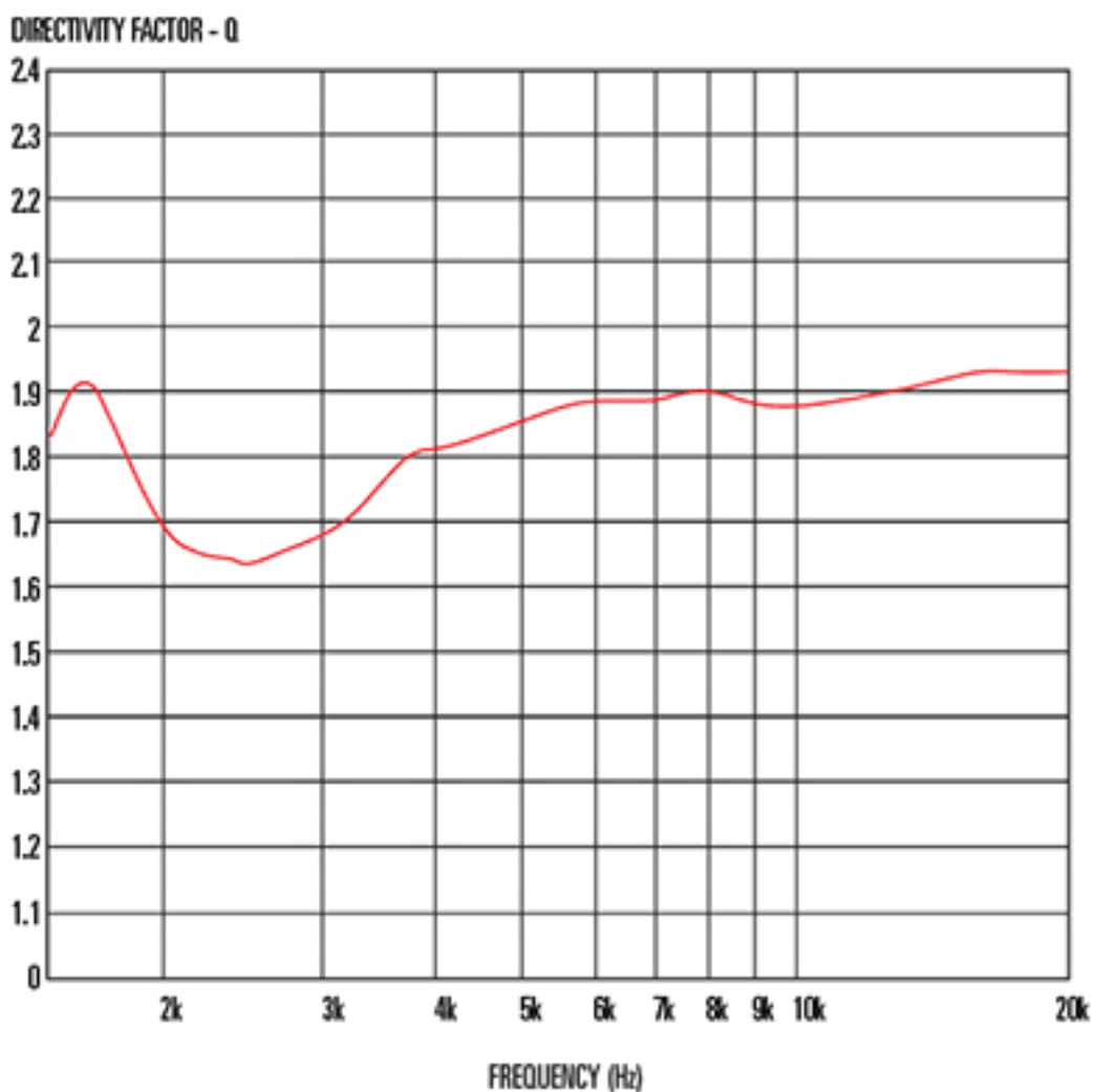
Directivity Factor
