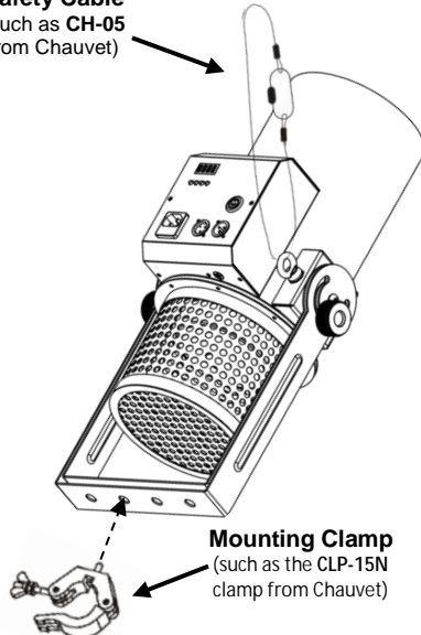
Overhead Mounting
